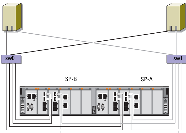
Almacenamiento Dell/EMC CX4-480 Fibre Channel
