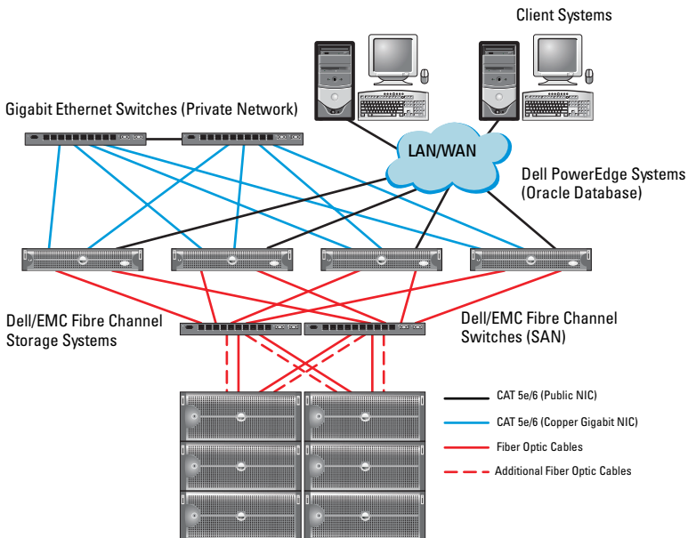
Figure 2-1. Hardware Connections for a SAN-Attached Fibre Channel Cluster
